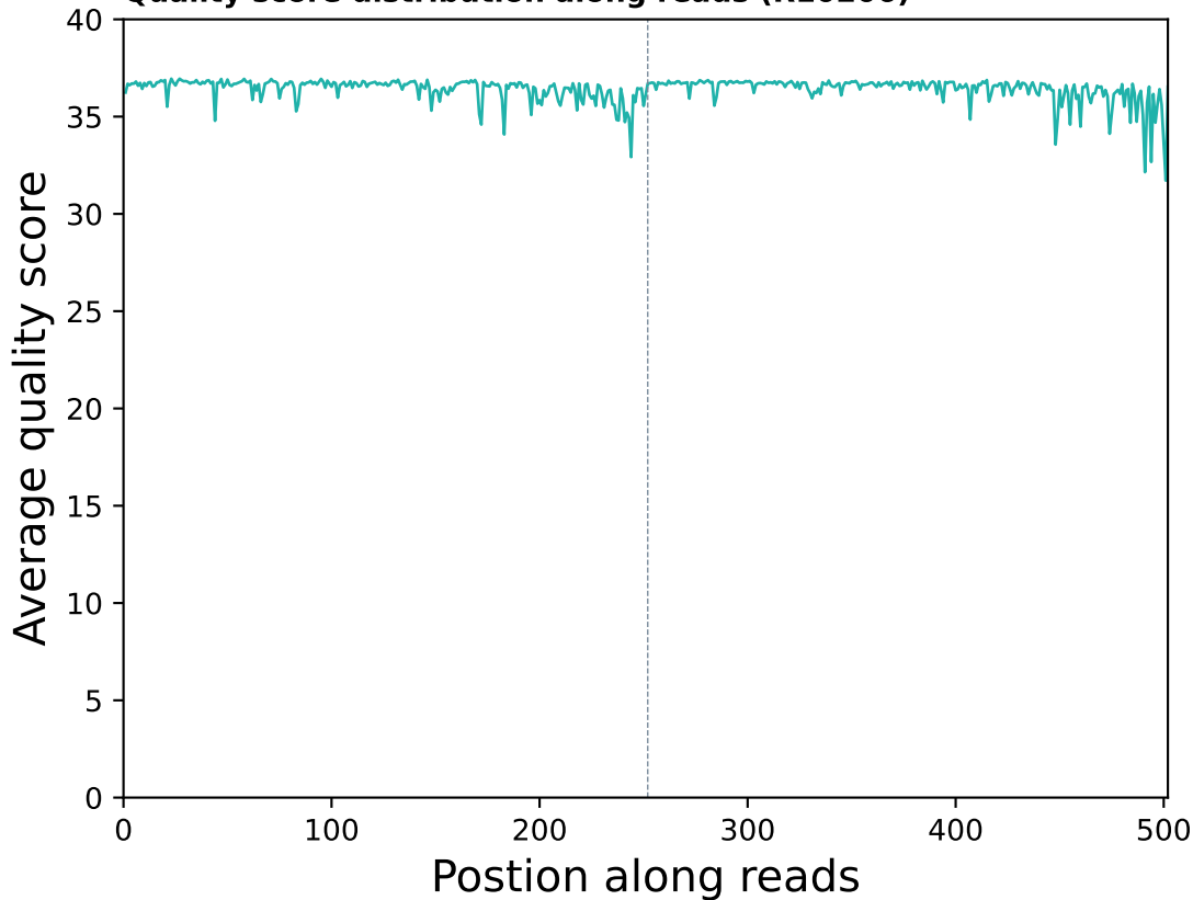
Quality score distribution along reads (R10206)
